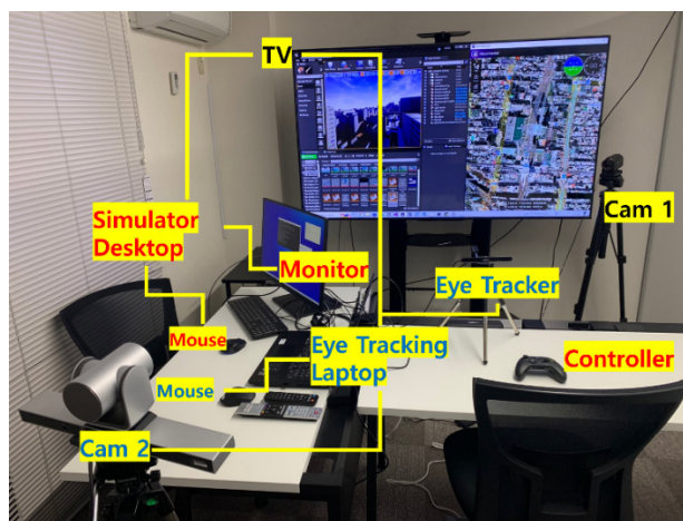
Fig. 3 Experimental setup featuring eye tracker, simulator, and cameras.
